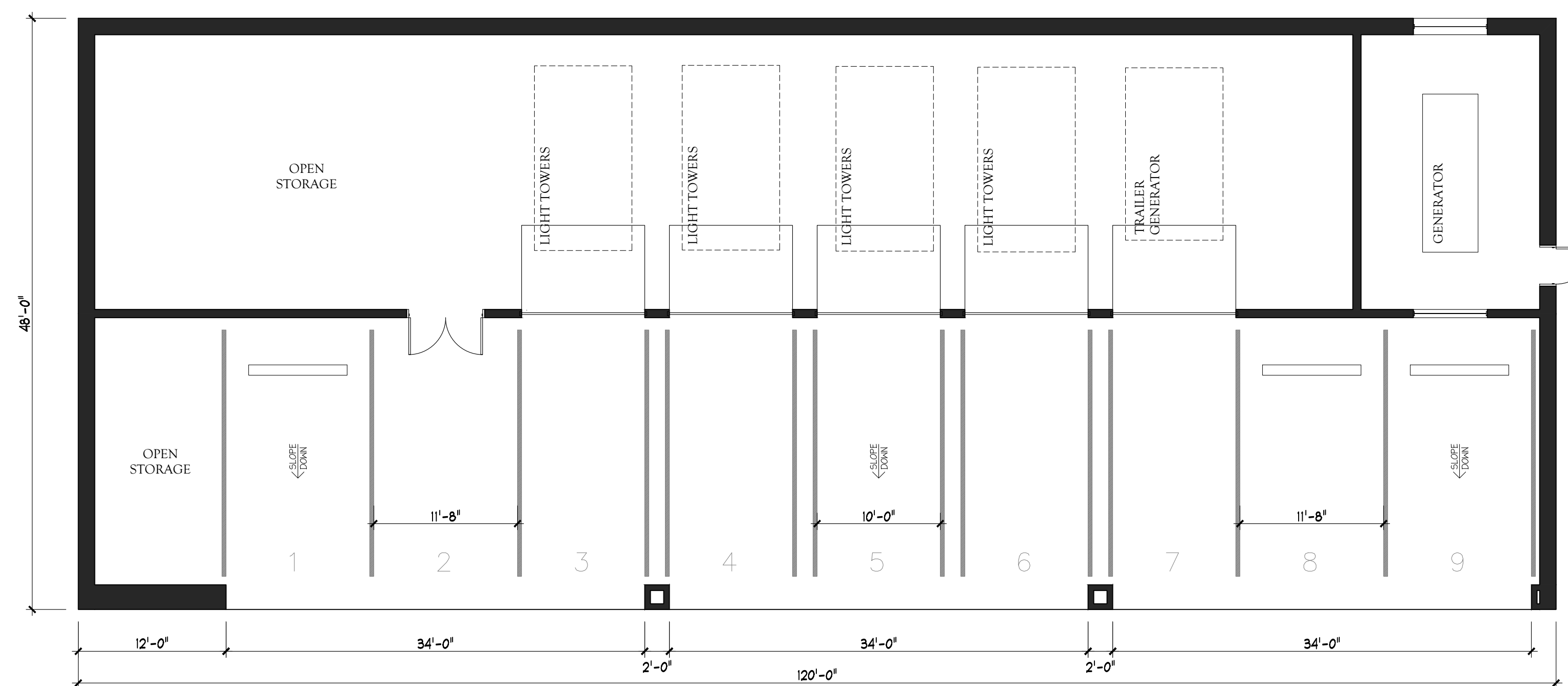
Proposed Outbuilding Plan
